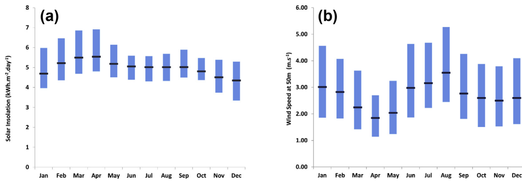
Fig. 6. (a) Maximum, minimum and monthly averaged solar insolation for Sarawak (data from NASA [70]); (b) Maximum, minimum and monthly averaged onshore wind speed (data from NASA [70]).
