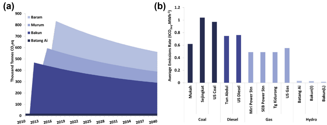
Fig. 8. (a) Results from IHA GHG assessment tool for SCORE dams; (b) Average emissions rate from various technologies.
