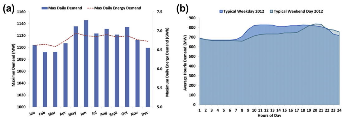
Fig. 3. (a) Monthly averaged and (b) Hourly averaged demand in Sarawak.
