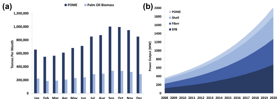
Fig. 4. (a) Estimates of palm oil waste availability based on monthly FFB processing; (b) Palm oil waste power potential based on future expansion (data from SEB [53]).
