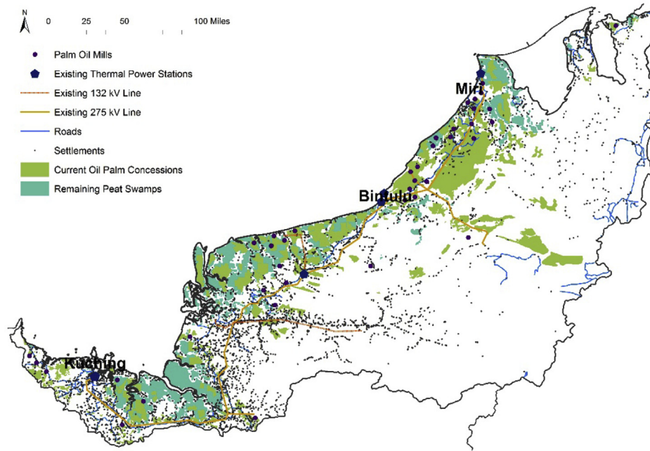
Fig. 5. Map of Sarawak showing current oil palm plantations and remaining peat swamp lands.
