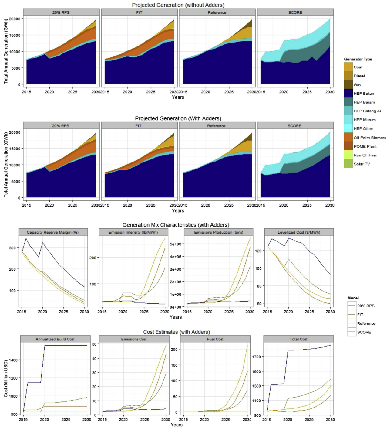
Fig. 9. Generation profile, cost components and generation characteristics of scenarios under 7% demand growth.
